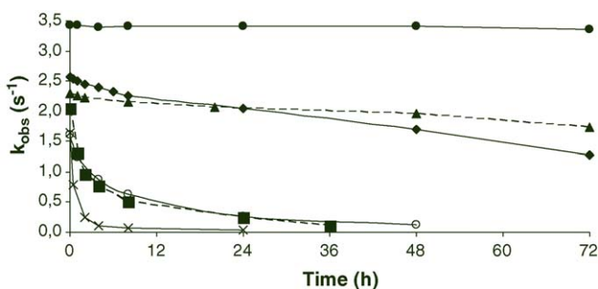
Fig. 3. PAMO stability in aqueous–organic media at 25 °C, 50 mM Tris/HCl pH 9 (●) or in buffer containing 10% (◆) or 30% methanol (▲), 10% (○) or 30% 1,4-dioxane, and 30% ethanol (×). The activity was measured at different times using phenylacetone as substrate.
