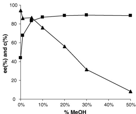
Fig. 1. Effect of methanol concentration on the degree of conversion (c) (▲) and on the ee of (R)-1a (■) in PAMO catalyzed oxidation of thioanisole (1). Reaction time: 24 h.
